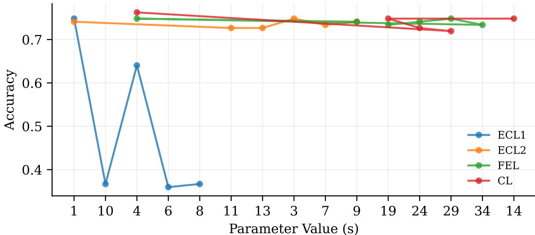
Parameter S Sensitivity Across Layers
